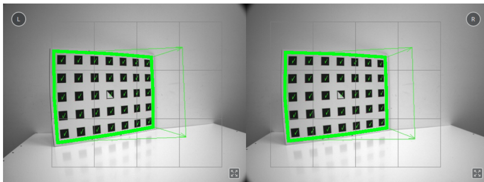
Fig. 6.32: Arrows indicating that the grid is not perpendicular to the camera's line of sight during stereo calibration
