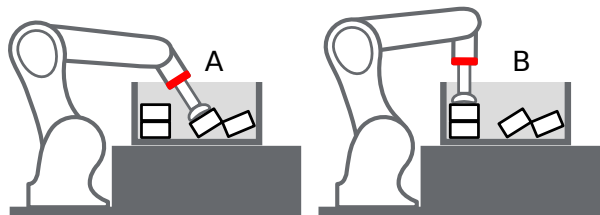
Fig. 6.44: Case A would be marked as collision only if check_flange is true, because the robot's flange (red) is inside the load carrier. Case B is collision free independent of check_flange .
