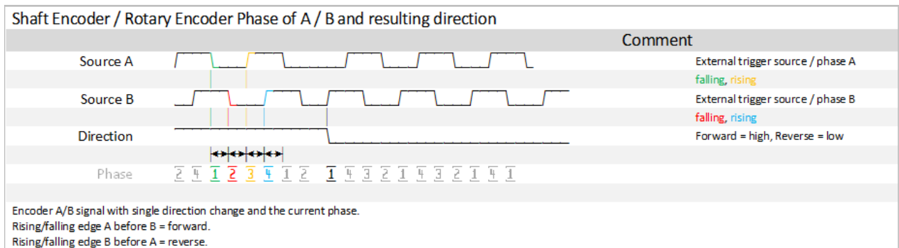
Figure 7.1. Shaft Encoder, A & B phase, direction
