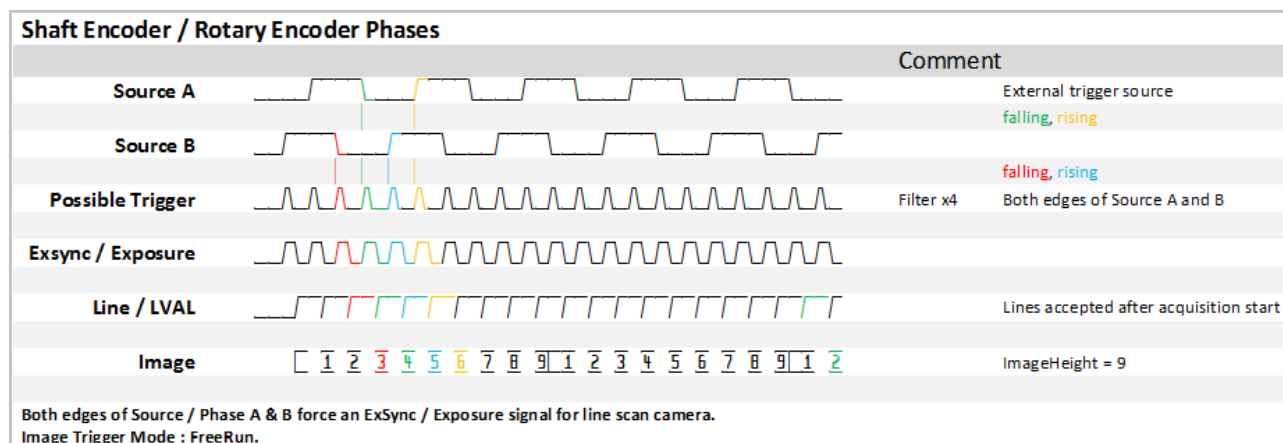
Figure 7.2. Shaft Encoder, A &amp; B signal, acquisition
